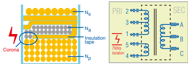
Primary winding fail cause insulation failure
